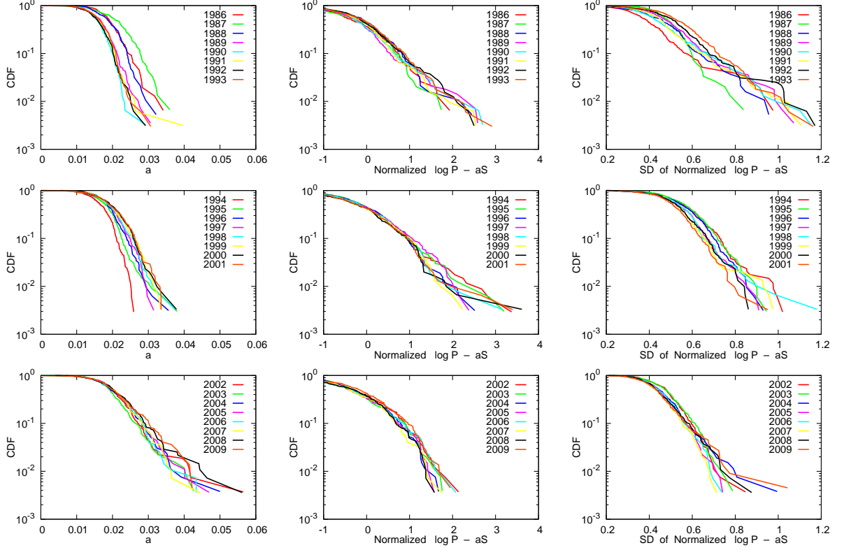
Figure 9: Dispersion of a_r , b_r and \sigma_r across pixels
